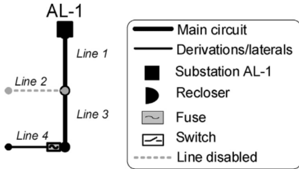
Fig. 7. Single-line diagram of the 4-bus reduced distribution system.
