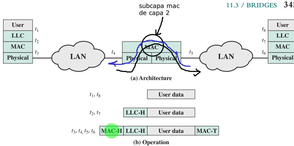
Figure 11.7 Connection of Two LANs by a Bridge
