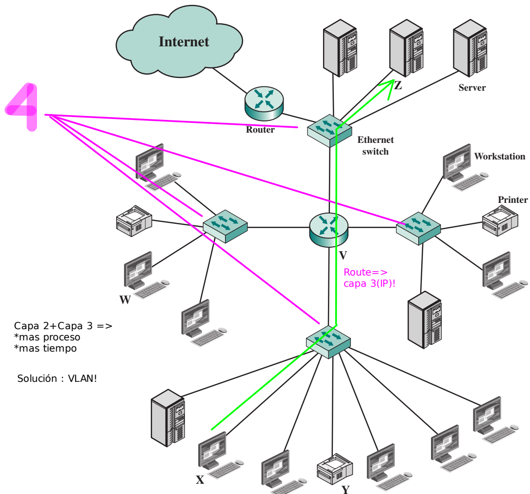
Figure 11.13 A Partitioned LAN
