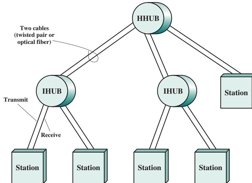
Figure 11.10 Two-Level Star Topology
