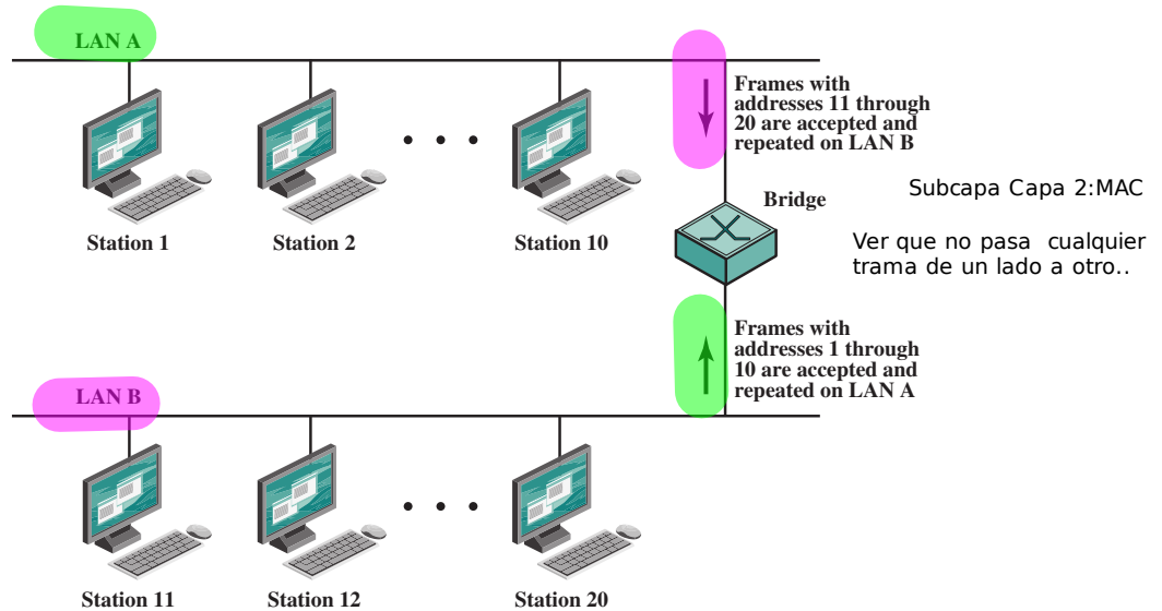
Figure 11.6 Bridge Operation
